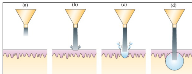
Figure 3. Mechanism of a liquid injection [6]
